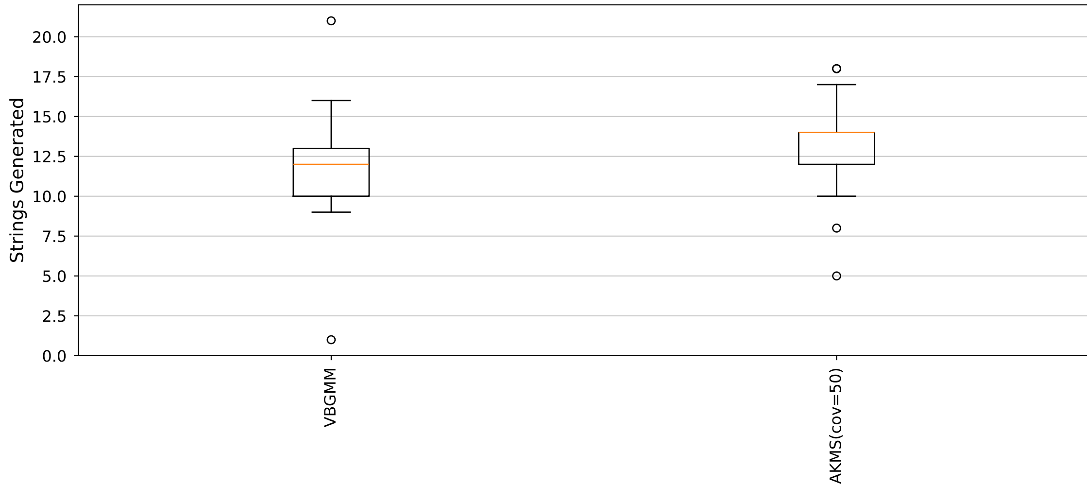
YARA Rules Strings Generated Distribution (Cluster17_Size8 dataset)
